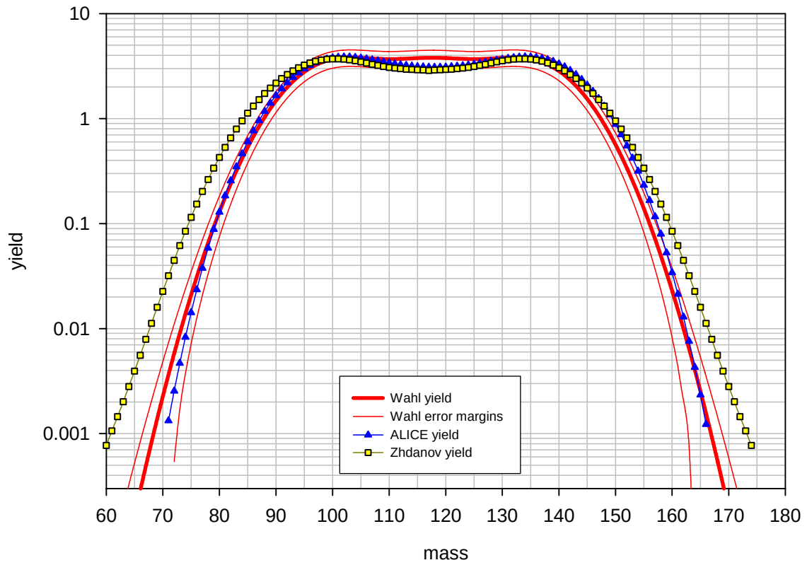
Benchmark B: ^{237}\text{Np} at 50 MeV, pre-neutron emission mass distribution
